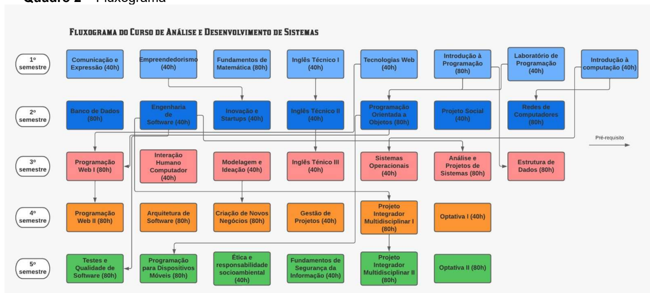
Quadro 2 – Fluxograma
